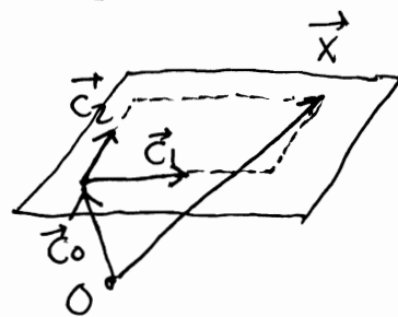
2-plane displaced from origin in \mathbb{R}^4
